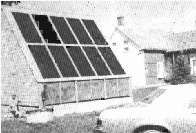
Dugald's solar collector
